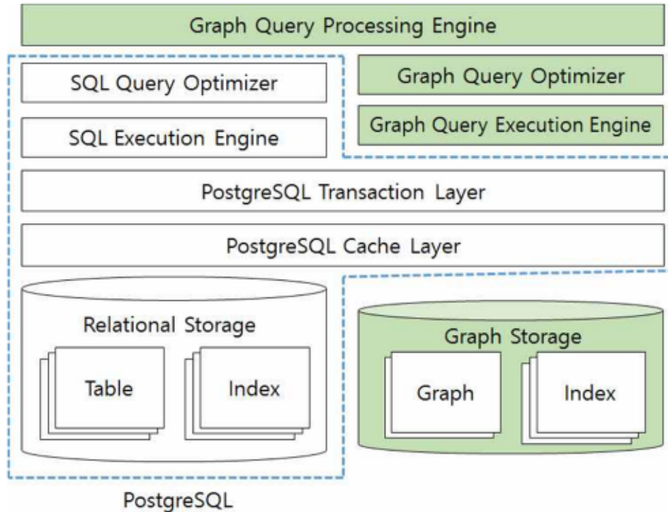
Figure 1: AgensGraph Architecture
