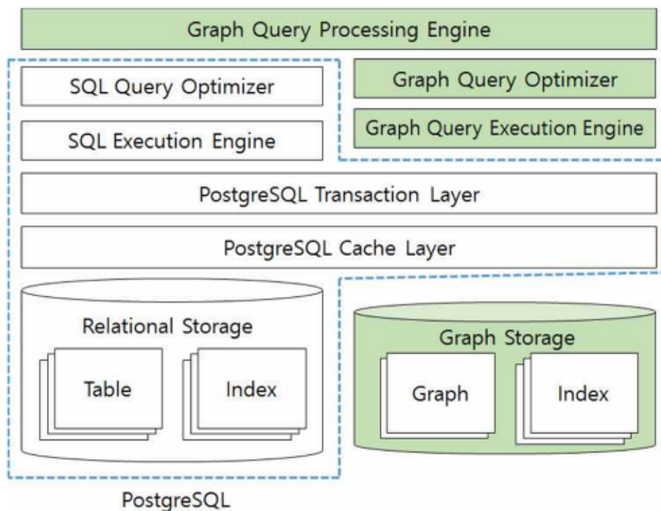
Figure 1.1: AgensGraph Architecture
